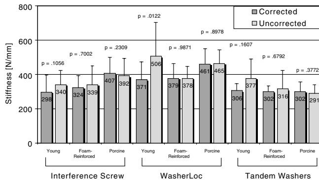
Figure 7. The corrected and uncorrected stiffness for the 3 tibial fixation devices tested in the 3 types of bone (mean ± 1 SD).
