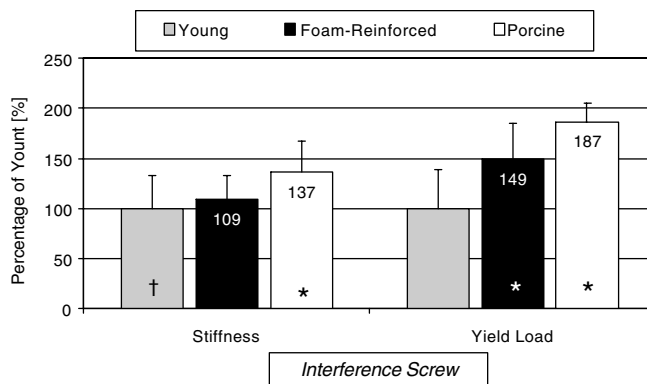
Figure 4. The normalized stiffness and yield of fixation with the interference screw in young human, foam-reinforced, and porcine tibiae. The asterisk (*) indicates that the fixation property in that type of bone was greater than that in young human tibiae ( P < .05 ). For fixation with the interference screw, stiffness and yield in foam-reinforced tibiae were more similar to those in young human tibiae than those in the porcine tibiae. The stiffness of the fixation with the interference screw in young human tibiae may have been less than 298 N/mm (†) because 2 of 7 specimens failed below the 350-N load increment, and these 2 specimens were excluded from the calculation of the average stiffness. Error bars indicate 1 standard deviation.
