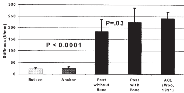
FIGURE 2. Stiffness comparison of four femur-fixation-DLSTG graft complexes to the native ACL. The stiffnesses of the femur-button-DLSTG graft complex and the femur-anchor-DLSTG graft complex were the same because the suture loop was the most elastic component. The stiffness of the femur-post without bone-DLSTG graft complex and the femur-post with bone graft-DLSTG graft complex were significantly greater than the stiffness of the femur-button-DLSTG graft complex and the femur-anchor-DLSTG graft complex with the button and anchor ( P < .0001 ). Compaction of bone graft into the femoral tunnel between the post and DLSTG graft significantly increased the stiffness 41 N/mm ( P = .03 ). The stiffness of the native ACL from young specimens is provided for comparison.
